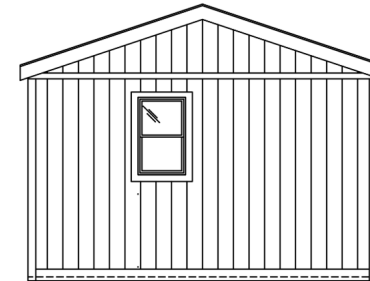
REAR ENDWALL
